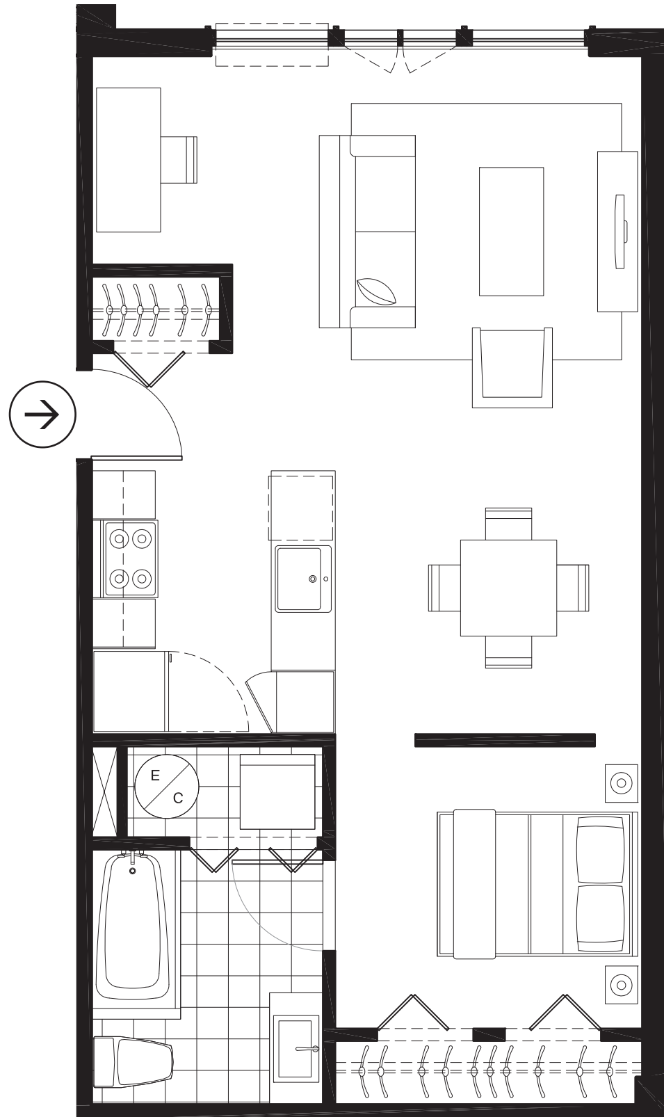
cuisine | kitchen 7'-7" x 8'-3" salle à manger, salon et bureau | dining room, living room & office room 17'-3" x 21'-2" chambre | bedroom 9'-7" x 8'-10" salle de bain | bathroom 7'-3" x 8'-0"
